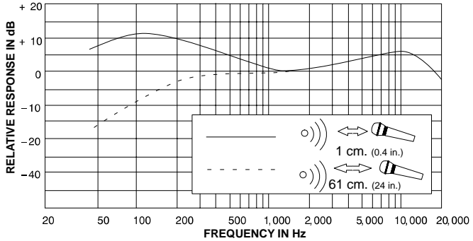
FIGURE 6. WH30: TYPICAL FREQUENCY RESPONSE
